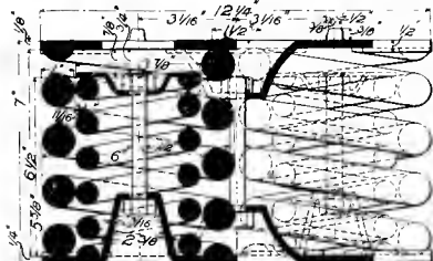
BOLSTER-SPRING, SEATS AND CAPS. NORFOLK & WESTERN RAILROAD. The number of springs depends on capacity of car, each spring being capable of carrying about 10,000 lbs.
